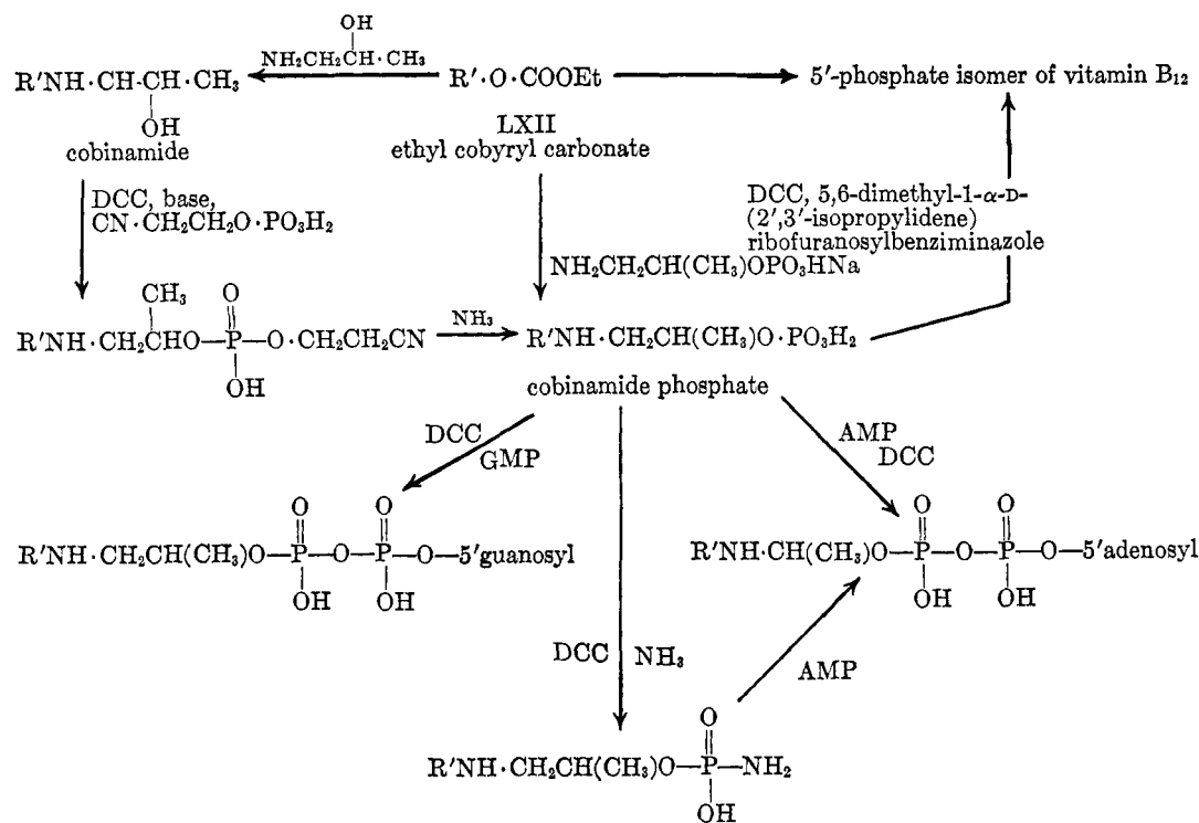
Fig. 15.—Some partial syntheses in the vitamin B 12 series (R' = cobyril, AMP = adenosine 5'-phosphate, GMP = guanosine 5'-phosphate, DCC = dicyclohexylcarbodiimide).
