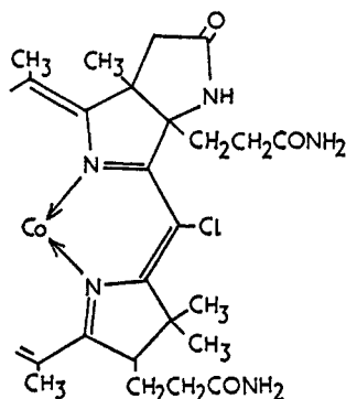
LVI. 8-Amino-10-chloro- \alpha -(5,6-dimethylbenziminazolyl)cobamic acid abdeg -pentamide c -lactam (partial structure, remainder as in vitamin B 12 ).
