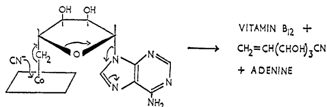
Fig. 12.—Cleavage of the coenzyme with cyanide ions.
