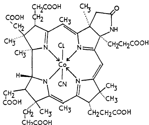
XV The hexabasic carboxylic acid
