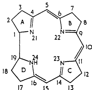
I. Corrin The basic ring system, indicating position numbering. Large letters denote individual pyrrole rings. C-20 is omitted; it becomes the \delta -carbon in the porphyrin nomenclature.
