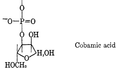
Fig. 1.—Nomenclature in the vitamin B 12 series.
